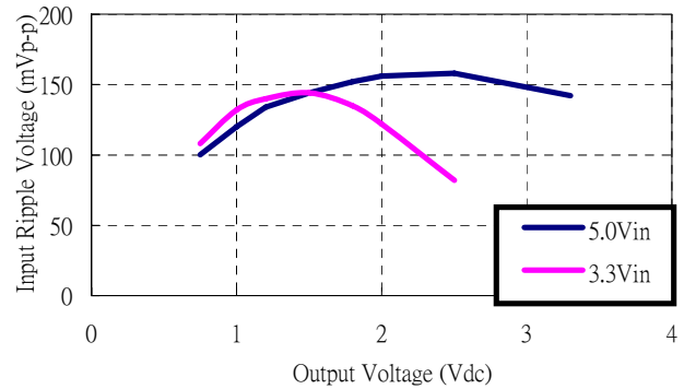
Figure 32: Input voltage ripple for various output models, IO = 10 A (CIN = 2x100 \mu F tantalum // 47 \mu F ceramic)
